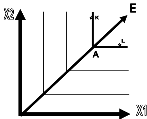
GRAPH I: Leontief Isoquants
